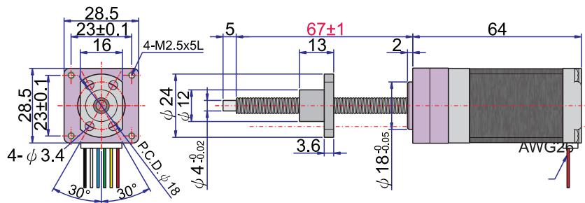
◆ MS225-09A-LSH0601
