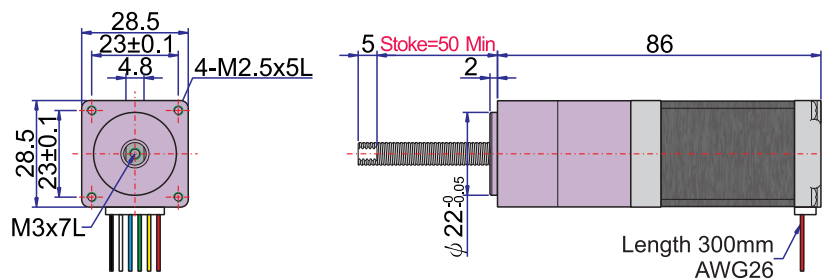
◆ MS225-09A-LNH0601
